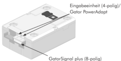
7.6.3 Gator 5000
